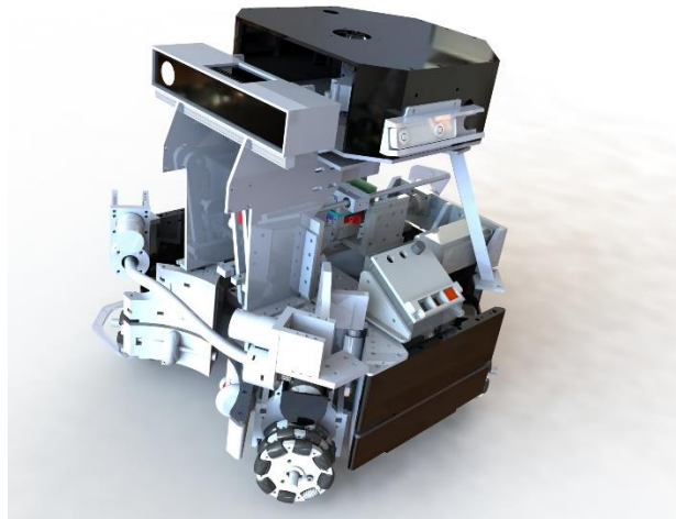
Fig. 1. Robot construction
